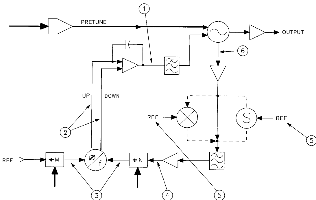
Figure 11-6. Unlocked PLL
